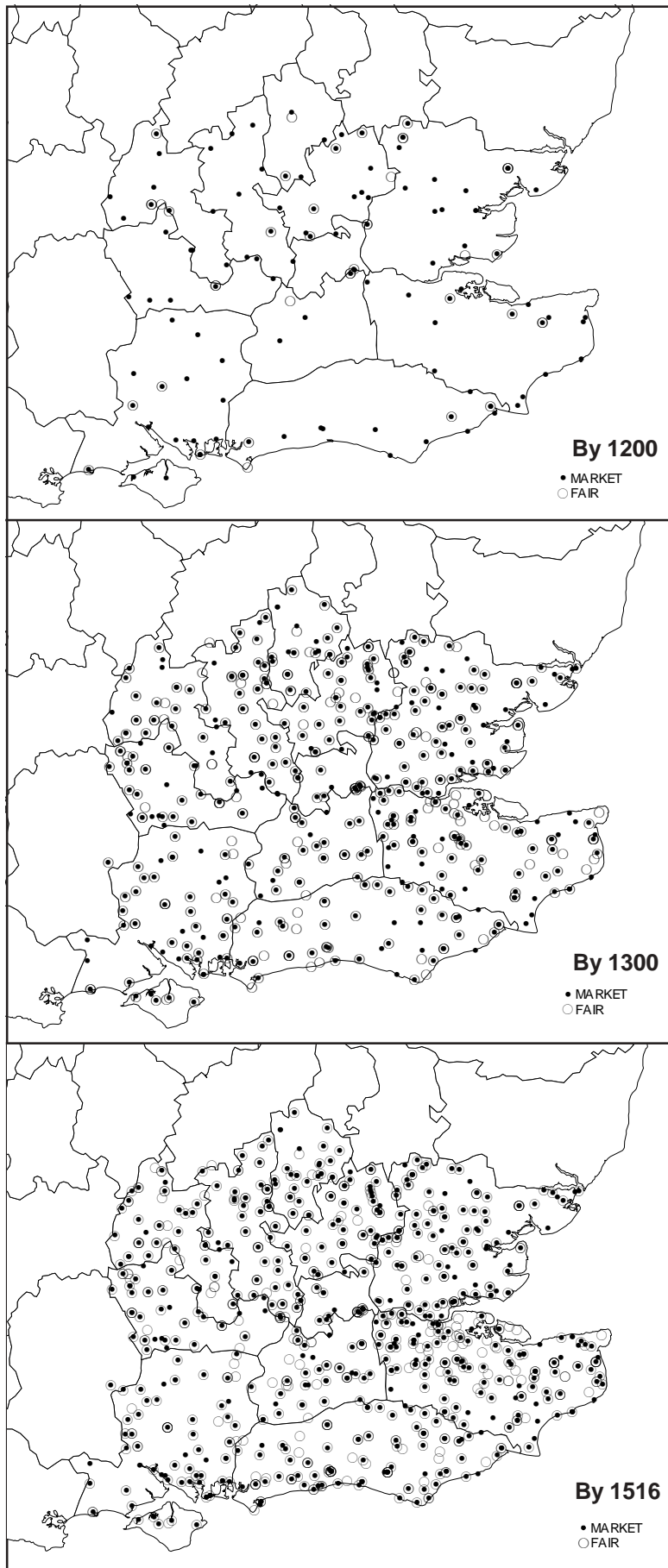
Fig. 4. Places in the South East with a market and/or fair by 1200, 1300 and 1516
